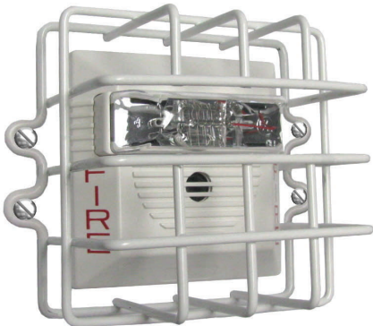
Guard pictured with Wheelock NS Series A/V Signal Appliance Fire Alarm
